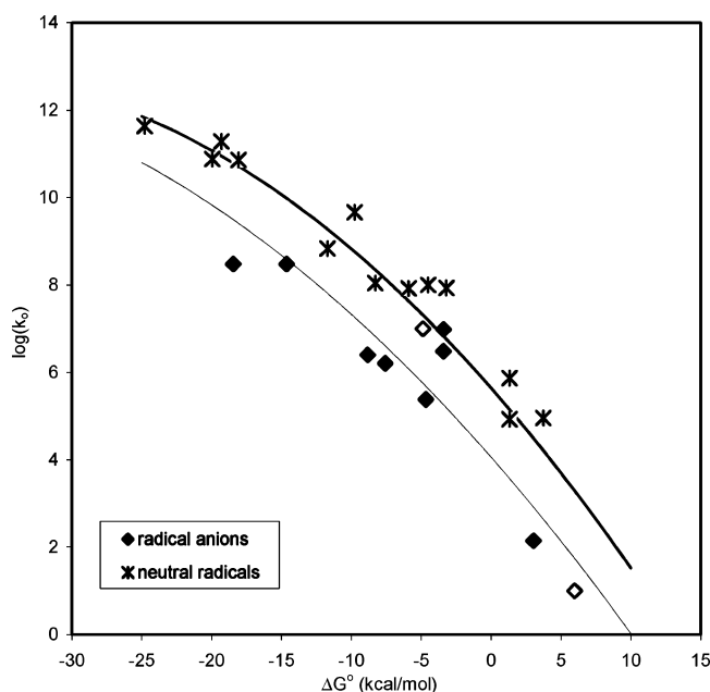
FIGURE 2. Structure/reactivity relationships for the cyclopropylcarbinyl \rightarrow homoallyl-type rearrangement of radical anions generated from carbonyl compounds and neutral free radicals (unshaded data points are based upon estimates of k_o ).
